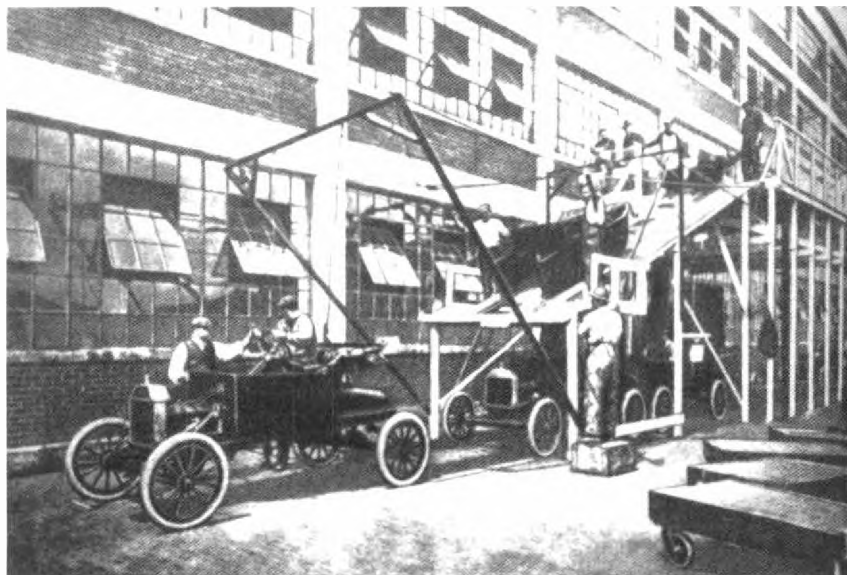
Ford zavodida avtomobillar yig'ish
